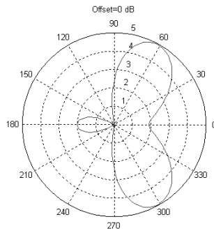
Figure 3(a): End-fire array with N=2 , Phase shift = -2\pi/3 , d = \lambda/3 , f = 75\text{MHz}
